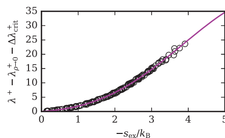
Figure 18. Scaled residual thermal conductivity data from the primary data sets 57,63–65 considered in the development of the correlation and the correlation from eq 65. Each marker corresponds to a single data point.
