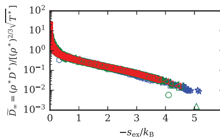
Figure 3. Rosenfeld-scaled self-diffusion values from simulations 41,42,42,46–48,50–53,58,59,69–71 for the Lennard-Jones 12-6 potential. Each marker/color pair is associated with a given data set. A larger version of this figure is available in the SI (Figure S3), along with a legend describing each data set.
