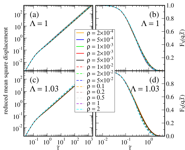
FIG. 9. (a) and (c) The reduced mean-square displacements; (b) and (d) intermediate scattering functions along the two isomorphs obtained from Eq. (25) for \Lambda = 1 (top) and \Lambda = 1.03 (bottom). Both sets of state points show almost invariant dynamics, although for \Lambda = 1.03 , the collapse is slightly worse than for \Lambda = 1 . The reduced scattering vector was again \tilde{q} = 7 .
