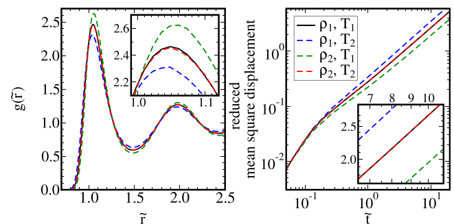
FIG. 2. The radial distribution function (left) and the mean square displacement (right) in reduced units for four different state points, two of which are isomorphous to each other. The initial state point (black line) has \rho_1 = 3 \times 10^{-3} , T_1 = 5.361 \times 10^{-5} , while the isomorphous state point (dashed, red line) has \rho_2 = 3.3 \times 10^{-3} , T_2 = 6.553 \times 10^{-5} . The method used to identify the state point ( \rho_2, T_2 ) as being isomorphous to state point ( \rho_1, T_1 ) is given below in Sec. IV A. The two isomorphous state points are seen to have identical structure and dynamics to a very good approximation. The effects of either changing density or temperature separately (green and blue dashed lines) are shown for comparison. The insets show enlarged views of the same data.
